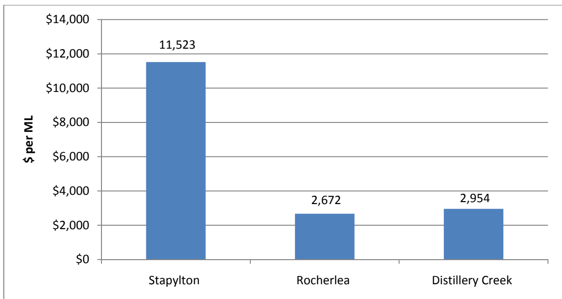
■ Figure 39 Comparison of operating expenditure per ML water storage capacity
