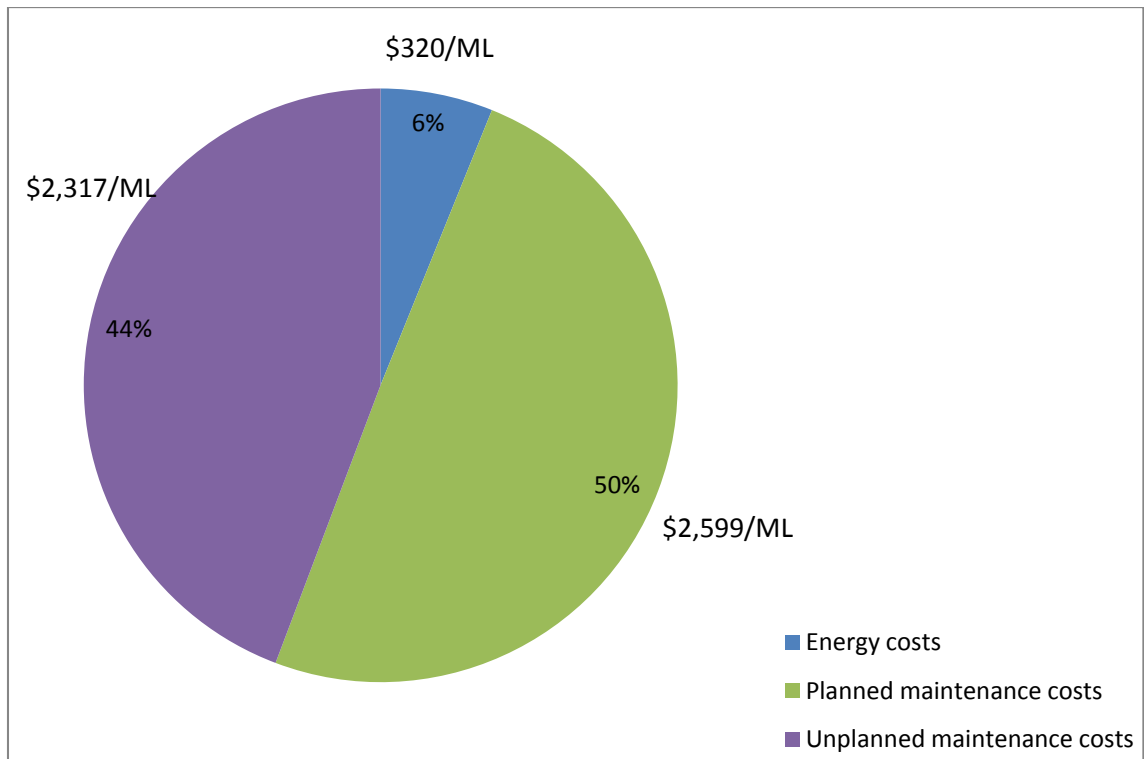
■ Figure 23 Percentage breakdown of operational costs per ML water treated for reservoirs
