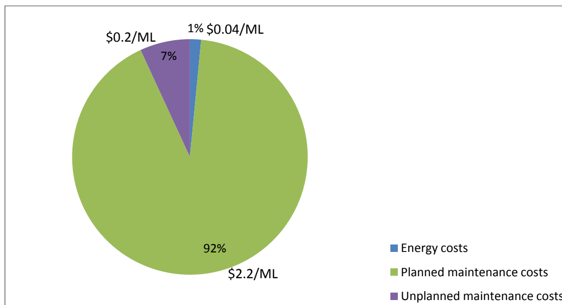
■ Figure 29 Percentage breakdown of operational costs per ML water transportation capacity for Bundamba Pump Station
