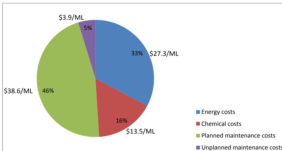
■ Figure 27 Percentage breakdown of operational costs per ML water treated for Chambers Flat Water Quality Facility
