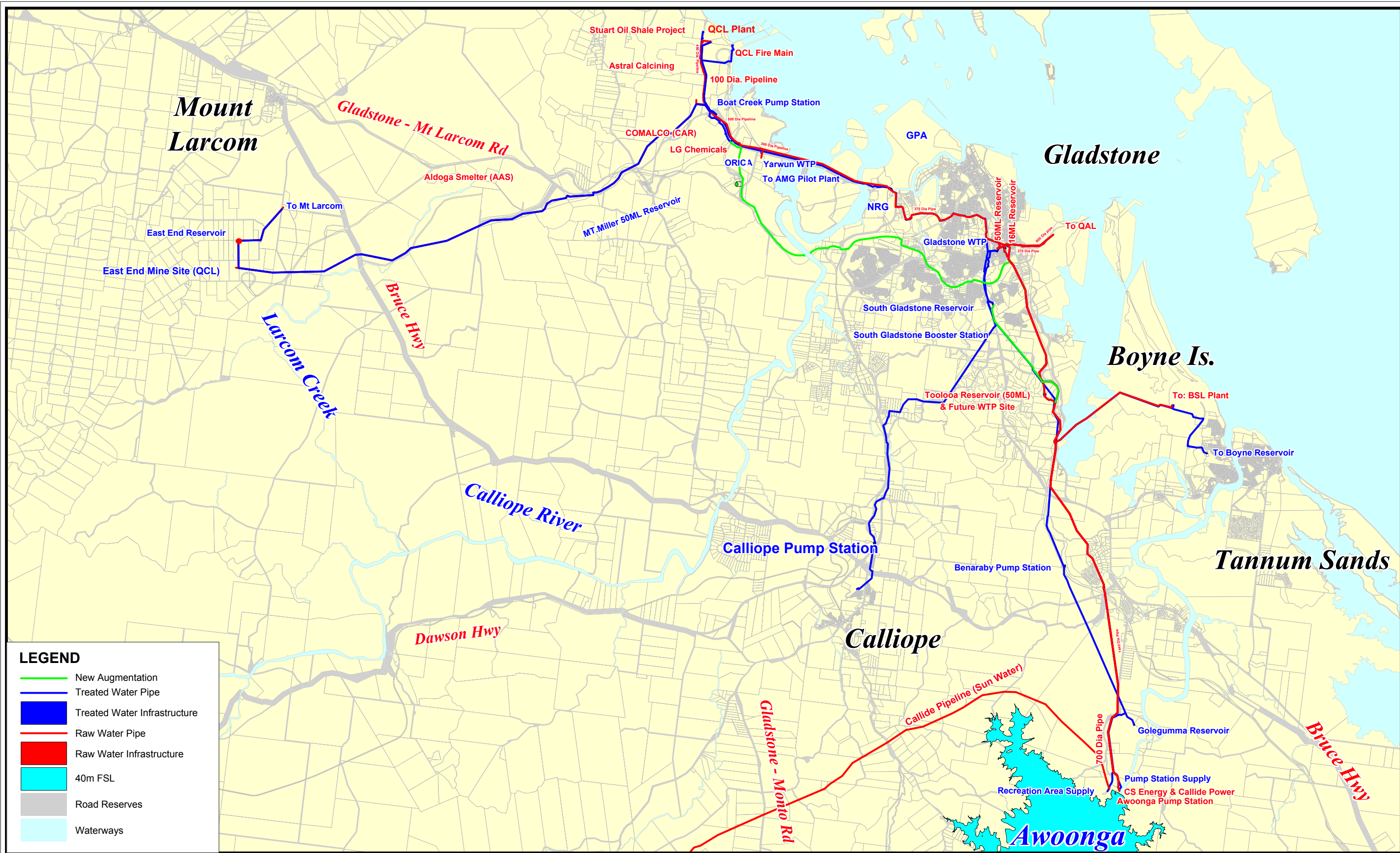
Figure 1: GLADSTONE AREA WATER BOARD WATER DELIVERY SYSTEMS
